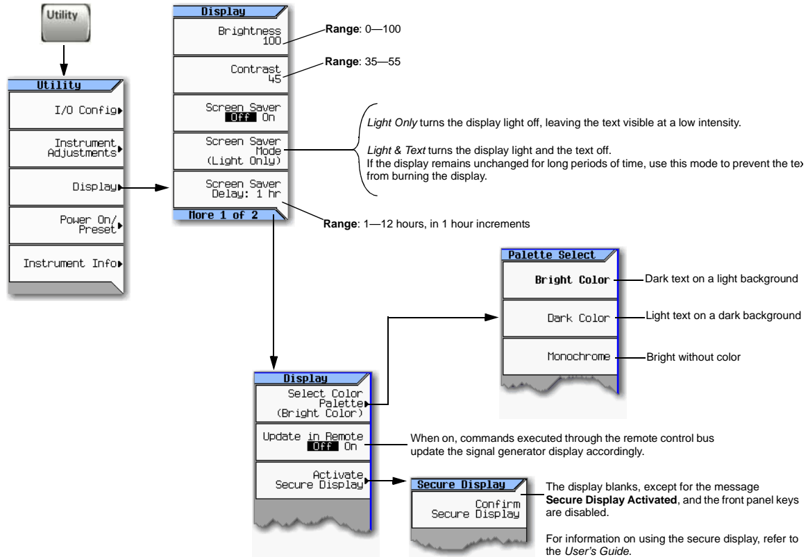
Figure 2-2 Display Softkeys
